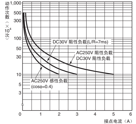
G2R-1Z、G2R-1AZ
